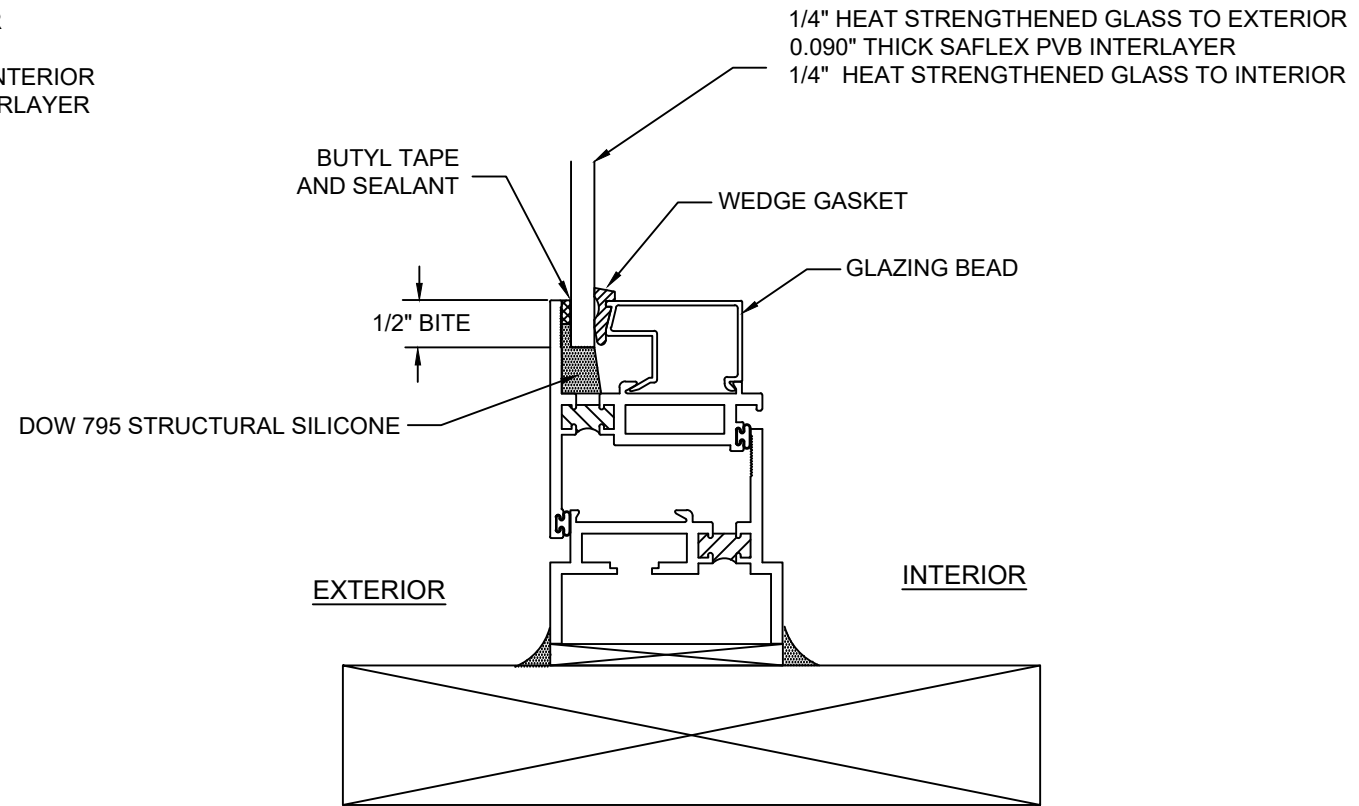
MONOLITHIC GLASS GLAZING DETAIL
