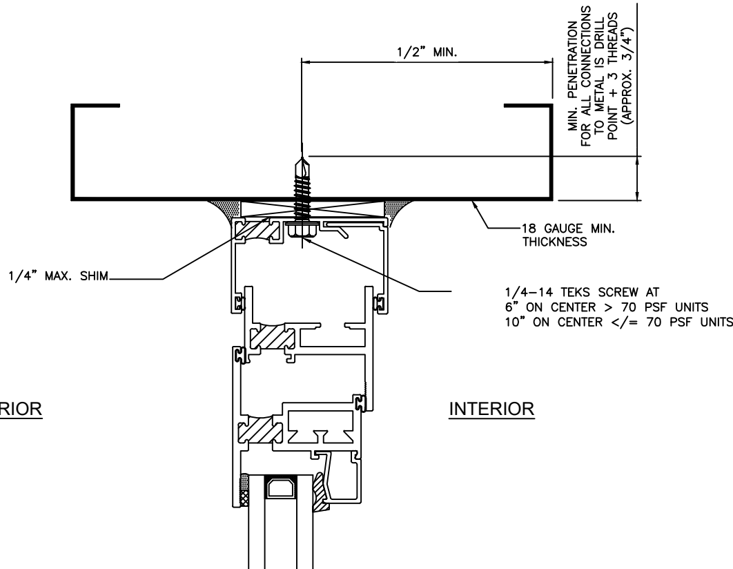
SECTION 1/1, 1/2 & 1/3 RECEPTOR TO STEEL STUD SUBSILL SIMILAR
