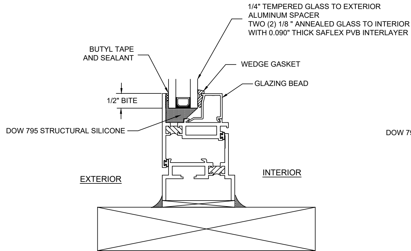
INSULATING GLASS GLAZING DETAIL
